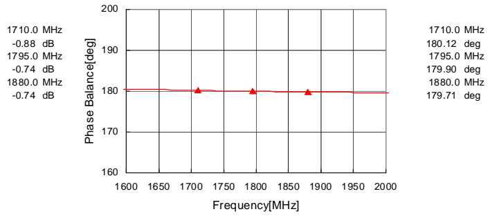
Phase Balance
